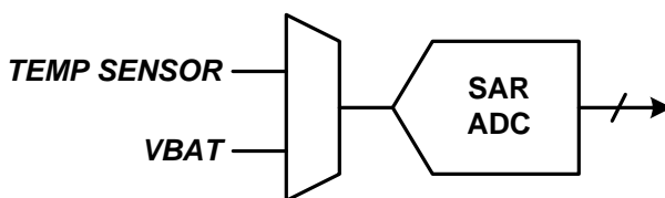
Figure 65. SAR Block Diagram
