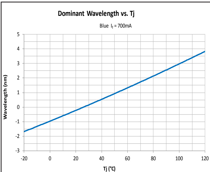
Relative Dominant Wavelength vs. Temperature - Blue
