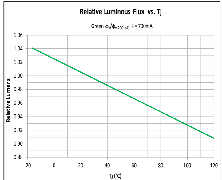
Relative Luminous Flux vs. Temperature - Green
