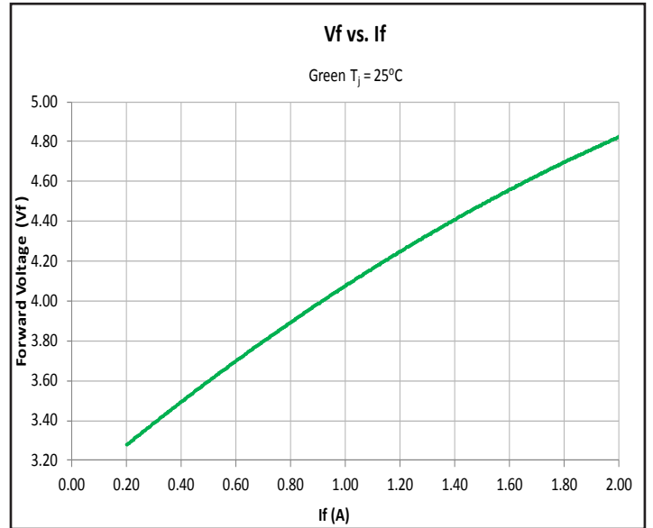
Voltage as function of Forward Current - Green
