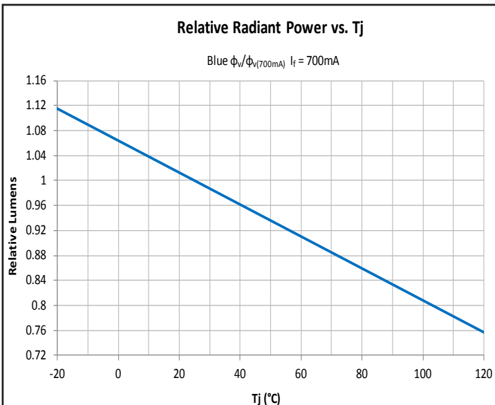
Relative Radiant Power vs. Temperature - Blue
