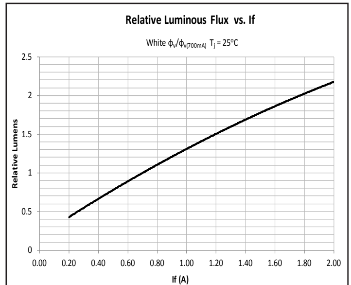
Relative Luminous Flux - White
