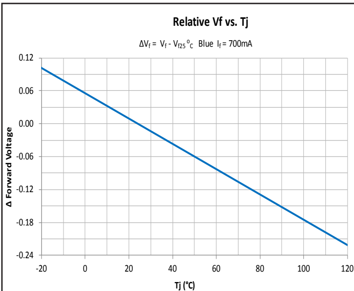
Relative Forward Voltage vs. Temperature - Blue
