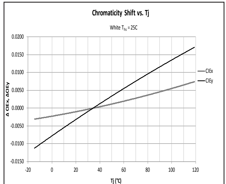
CIEx, y change vs. Temperature - White
