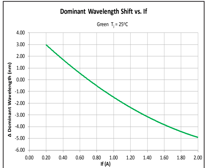
Wavelength change as function of Current - Green
