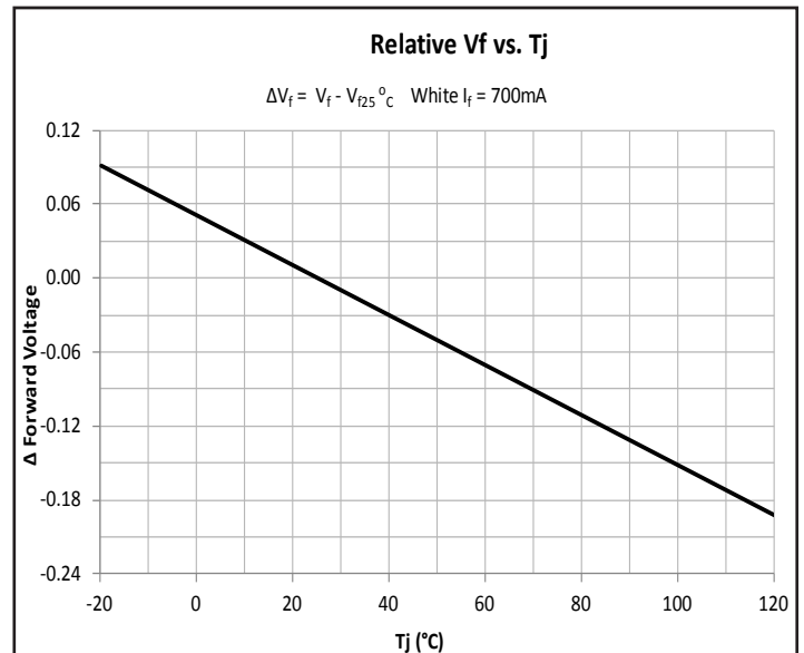
Relative Forward Voltage vs. Temperature - White
