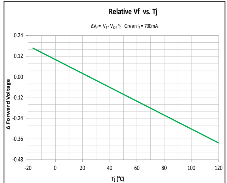
Relative Forward Voltage vs. Temperature - Green
