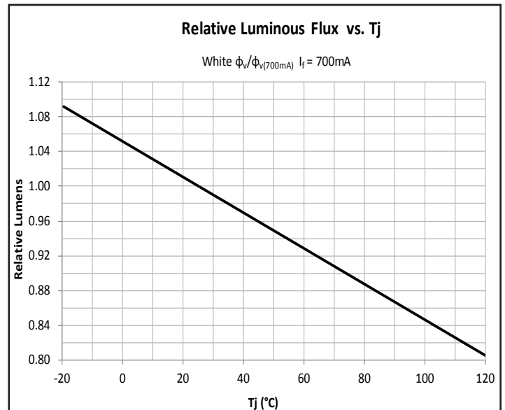
Relative Luminous Flux vs. Temperature - White
