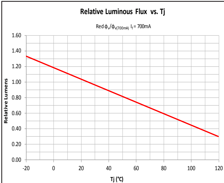
Relative Luminous Flux vs. Temperature - Red
