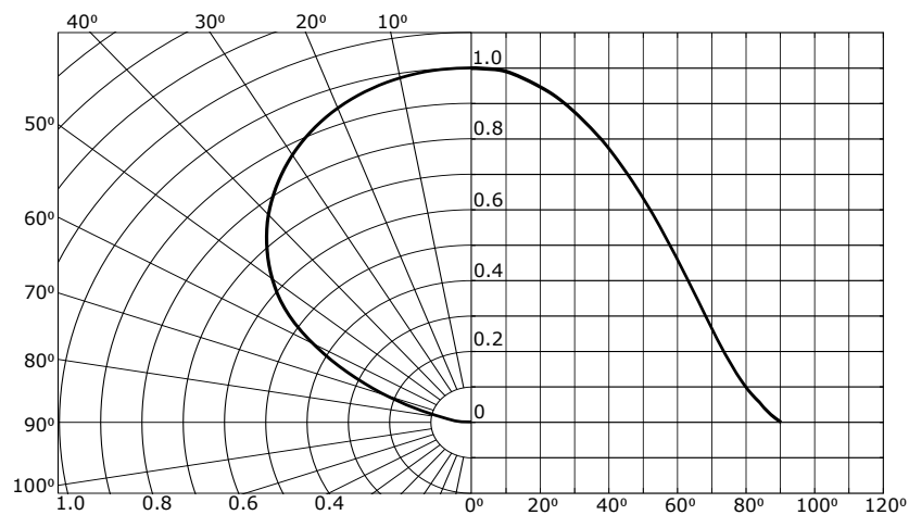
SBM-40-RGBW Angular Distribution
