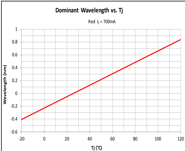
Relative Dominant Wavelength vs. Temperature - Red
