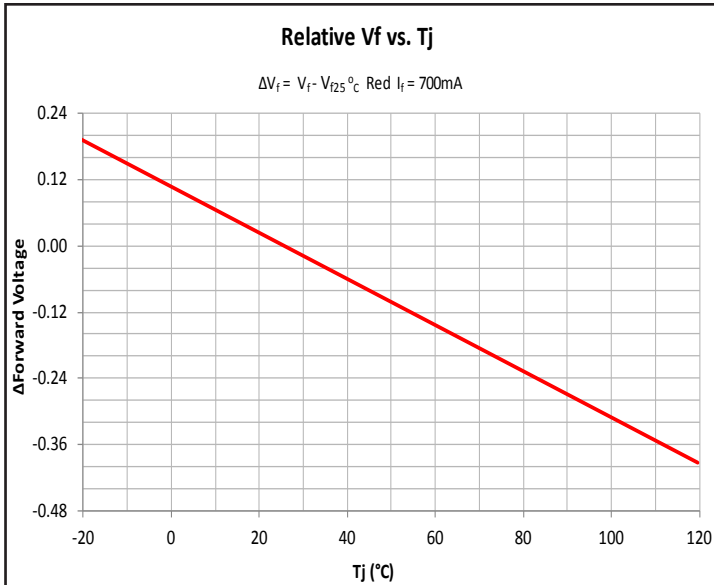
Relative Forward Voltage vs. Temperature - Red
