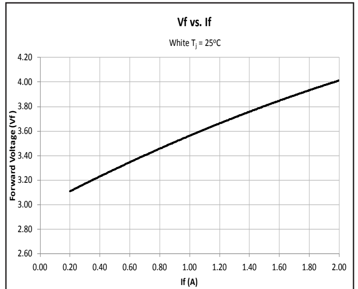
Voltage as function of Forward Current - White
