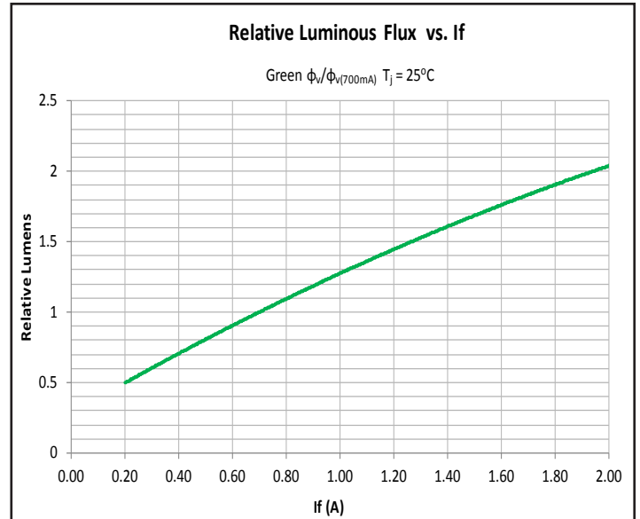
Relative Luminous Flux - Green
