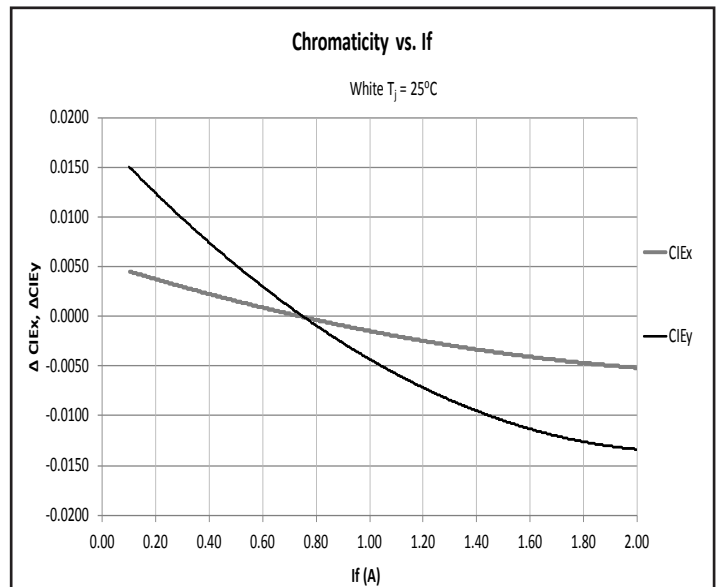
CIEx, y change as function of Current - White
